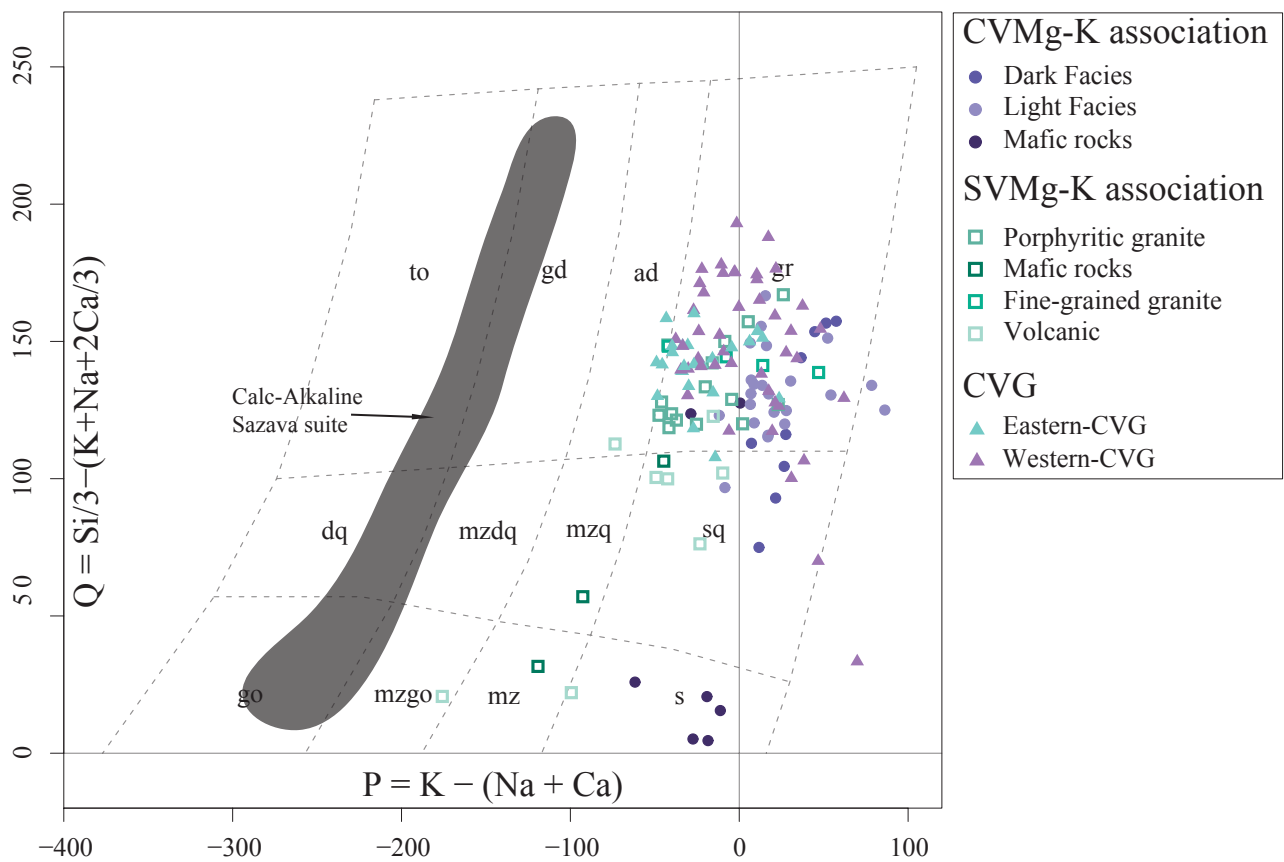
Figure 2: Multicationic P-Q plot (Debon & Le Fort, 1983) for granitoids of Vosges Mts; P represents the proportion of K-feldspar to plagioclase and Q the quartz content. The calc-alkaline Sázava suite from Bohemia (Janoušek et al., 2000) is plotted for comparison.
