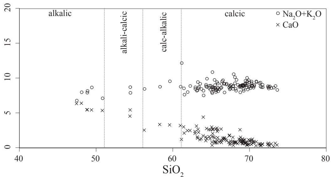
Figure 8: Variations of CaO wt% and \text{Na}_2\text{O} + \text{K}_2\text{O} vs. \text{SiO}_2 wt% for Vosgian rocks. Original named fields within \text{SiO}_2 wt% ranges are Peacock (1931) and are applied to suites whose oxide variation trends intersect within a given field.
