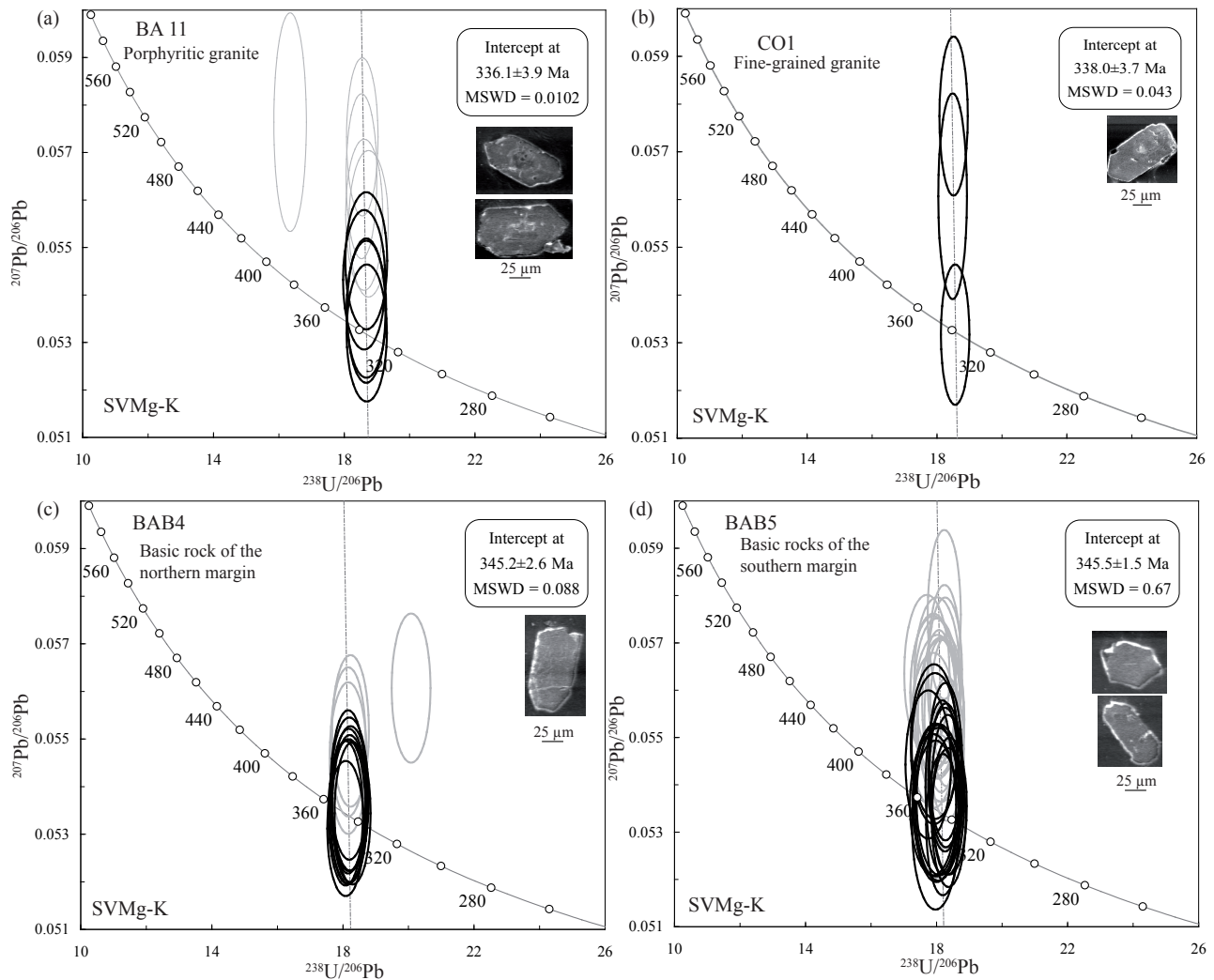
Figure 5: U-Pb concordia diagrams for SVMg-K.
