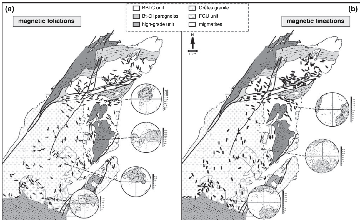
Fig. 6 Map of AMS fabric data of the southern domain and also of the BBTC intrusions. a Magnetic foliations. Contoured stereonet of poles to magnetic foliation ( k_3 direction) show the distribution of k_3 for northern, central and southern parts and the Crêtes granite; see discussion in the text (equal area, lower hemisphere projection, contoured at multiples of uniform distribution). b Magnetic lineations
