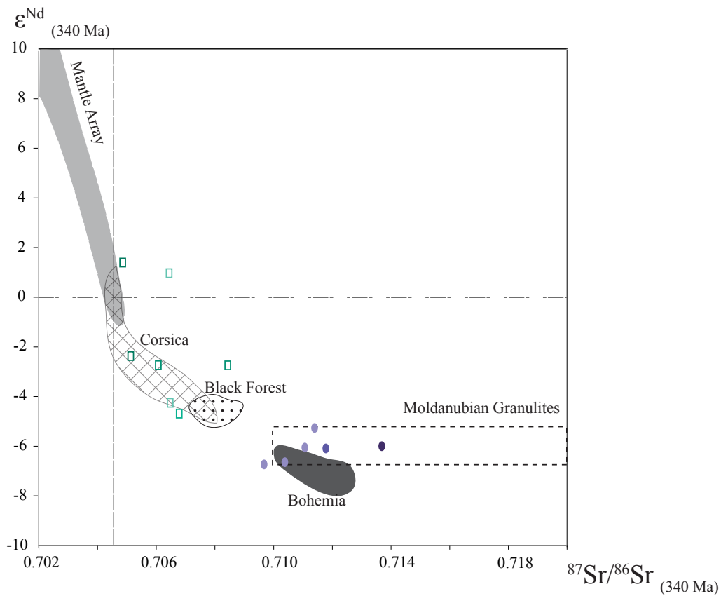
Figure 16: (^{87}\text{Sr}/^{86}\text{Sr})_{340} vs. \epsilon_{\text{Nd}}^{340} plot for other Mg-K Variscan plutons. Data from Janoušek et al., 1995 and Holub and Janoušek, 2003 for Bohemian Massif, Schaltegger et al., 1991, Debon and Lemmet, 1999 and Debon et al., 1998 for External Crystalline Massifs of the Alps, Hann, 2003 and Schaltegger, 2000 for Black Forest and Rossi & Cocherie, 1991 and Cocherie et al., 1994 for Corsica Batholith. Mg-K Vosgian samples are plotted for comparison. Corsica, CVMg-K and Black Forest data as well as CVMg-K and Bohemia data are arranged in two independent clouds, suggesting a genesis from different protoliths. Same legend as Fig. 10.
