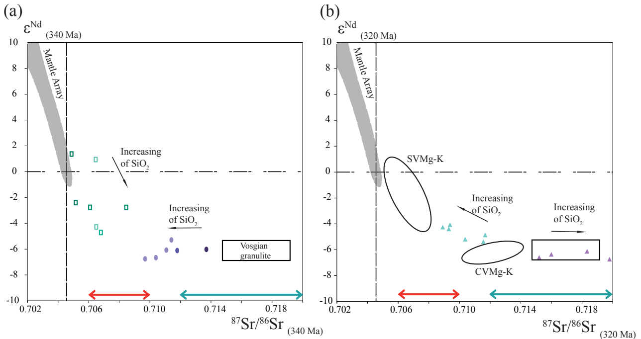
Figure 10: (a) (^{87}\text{Sr}/^{86}\text{Sr})_{340} vs. \varepsilon_{\text{Nd}}^{340} plot for SVMg-K and CVMg-K. Arrows show trend from mafic to felsic end-members for the two associations. (b) (^{87}\text{Sr}/^{86}\text{Sr})_{320} vs. \varepsilon_{\text{Nd}}^{320} plot for W-CVG and E-CVG; CVMg-K and SVMg-K fields are indicated for comparison. Red arrow represents ^{87}\text{Sr}/^{86}\text{Sr} of Vosgian orthogneiss (Bonhomme & Fluck, 1981) and green arrow represents ^{87}\text{Sr}/^{86}\text{Sr} of Vosgian granulite and paragneiss recalculated at 340 Ma. Black rectangle represents isotopic composition of Vosgian granulite (Skrzypek, 2011). Same legend as Fig. 2.
