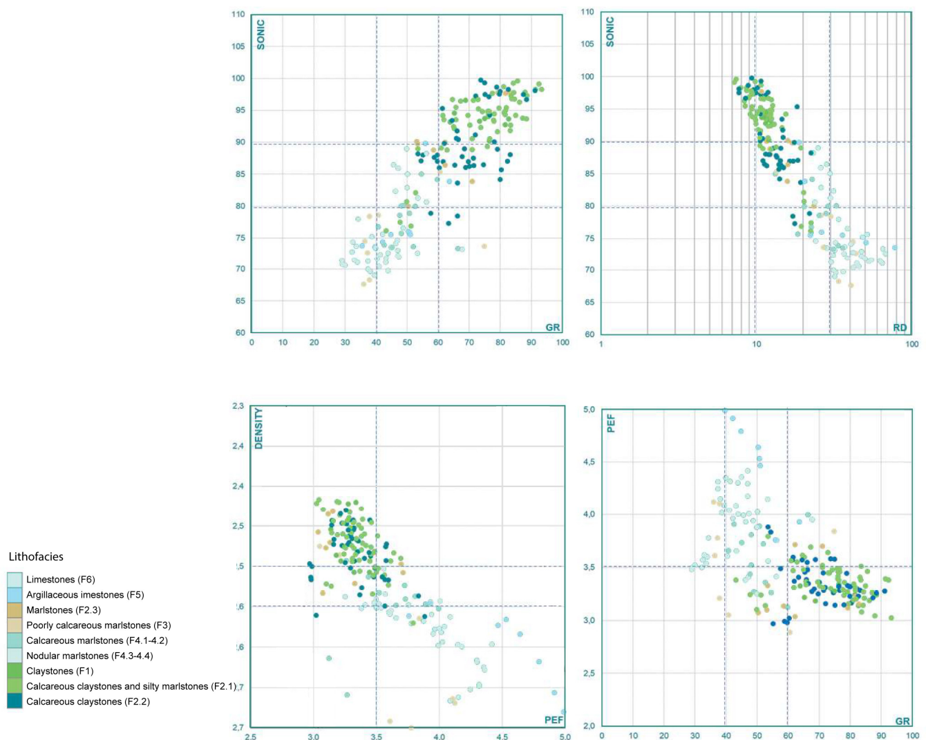
Figure 5. Diagrams in 3D showing the relationship between the wirelines' signals (x and y axes) and lithofacies descriptions (plotted by colour). The DT (Sonic) and density values are well correlated and show redundant information with the GR and PEF values. The most discriminant wirelines for lithofacies determination are GR, DR and PEF.
