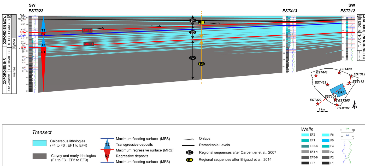
Figure 9. Correlations on an NE-SW transect (wells EST322 – EST413 – EST312) showing lithological evolution and transgression/regression cycles. Litho and electrofacies have been grouped into calcareous deposits (from nodular marlstone to massive limestone in blue) and clayey deposits (clays, silty calcareous clays and bioclastic marlstone in grey). Wells have been horizontalised on surface RL2.
