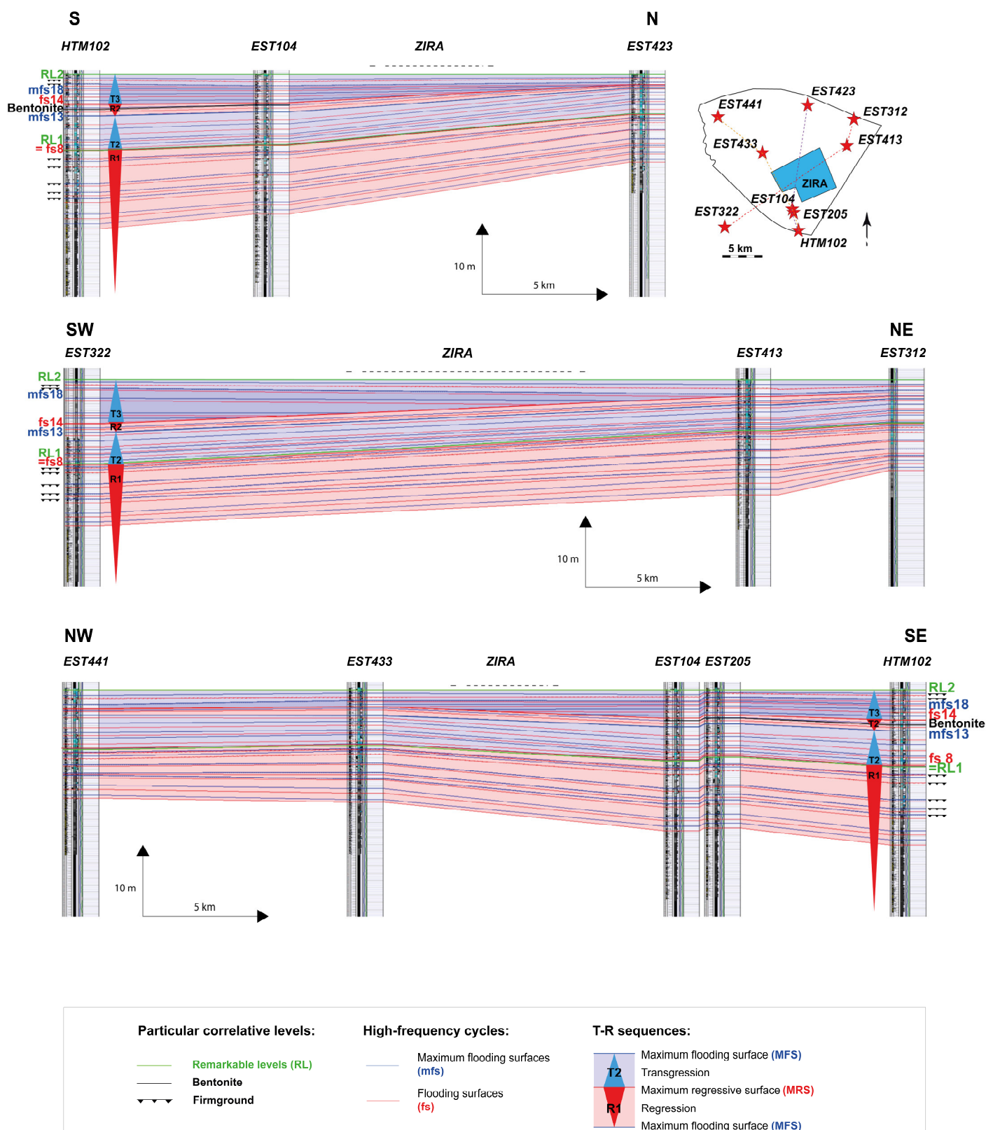
Figure 8. Correlation of the nine wells investigated around the ZIRA based on the main remarkable surfaces. Wells have been horizontalised on surface RS2.
