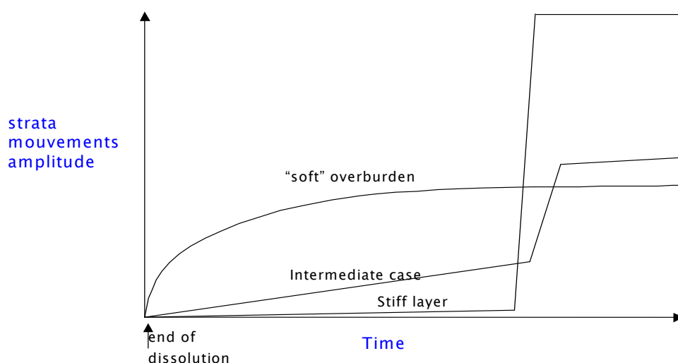
Figure 12 : schematic representation of the cavity evolution for different bedded salt contexts and induced soil movements.
