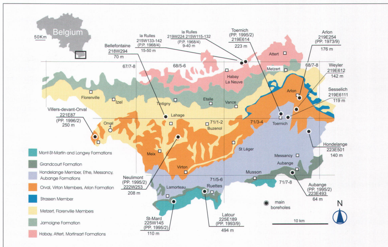
Figure 1. Simplified geological map of Belgian Lorraine.
