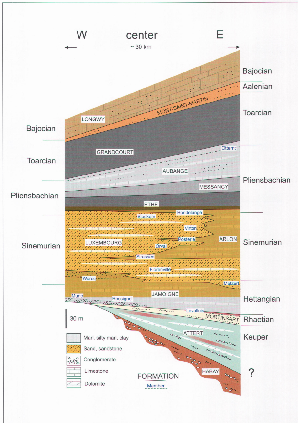
Figure 3. E-W schematic lithostratigraphic section of Belgian Lorraine.
